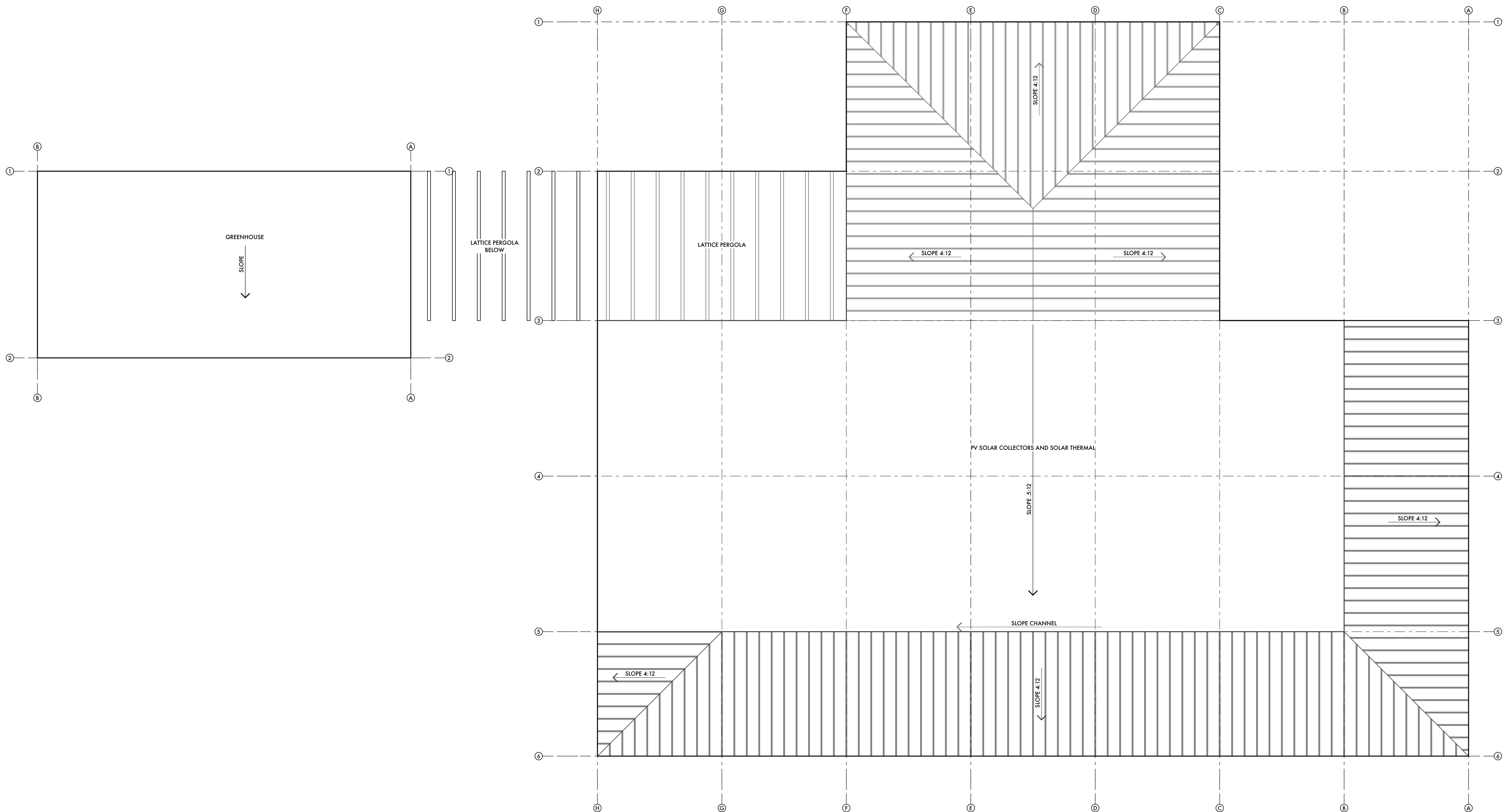
1 Roof Level WORKING Plan SCALE: 1/8" = 1'-0"
