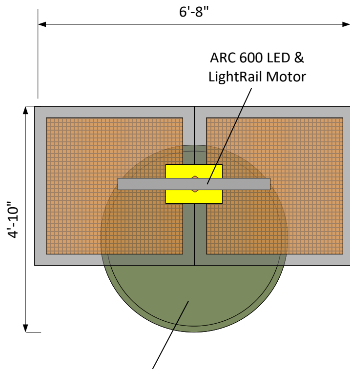
125 Gallon Fish tank Dia. 48", Depth 22"
